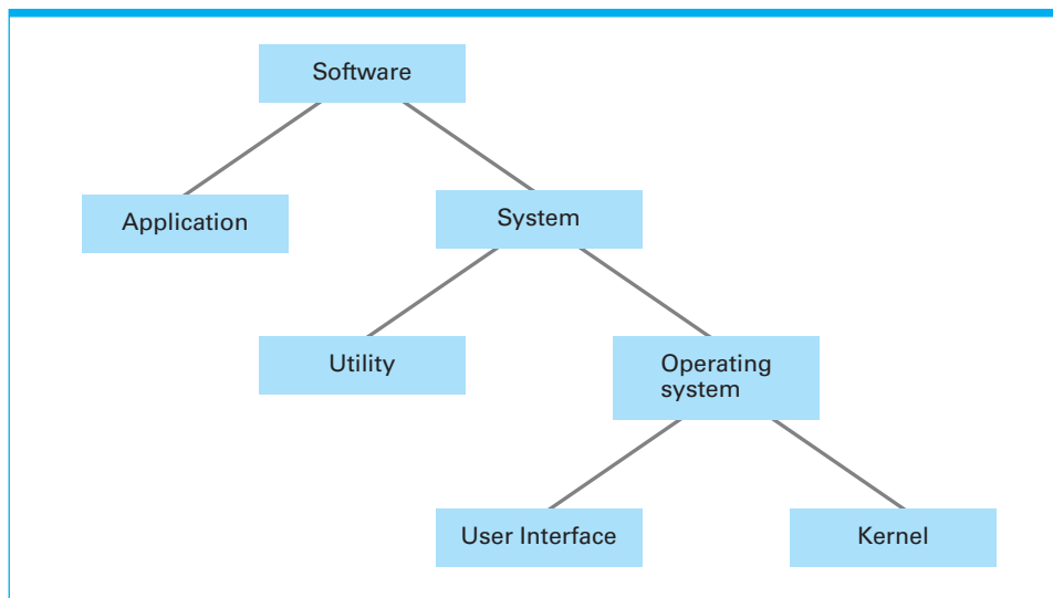
Figure 3.3 Software classification
