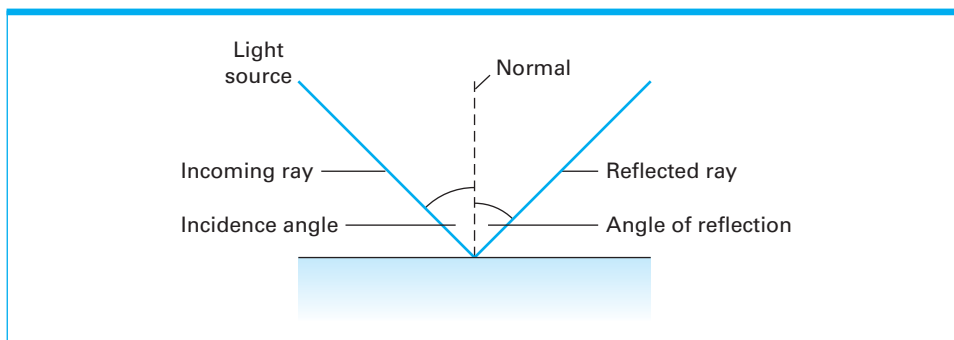
Figure 10.7 Reflected light
