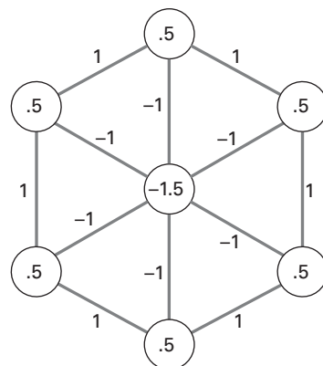
Figure 11.21 An artificial neural network implementing an associative memory
