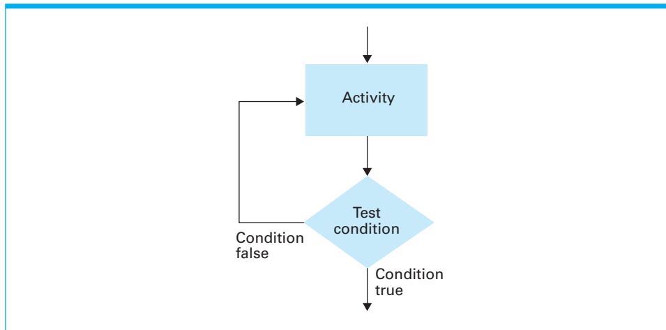
Figure 5.9 The repeat loop structure
