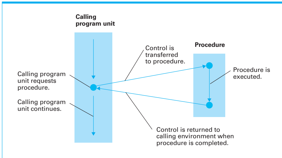
Figure 6.8 The flow of control involving a procedure
