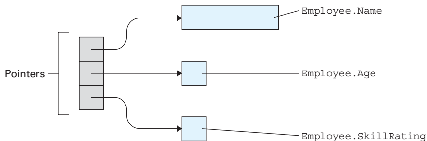
b. Array components stored in separate locations
