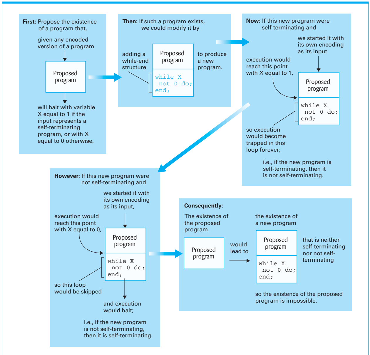
Figure 12.7 Proving the unsolvability of the halting problem
