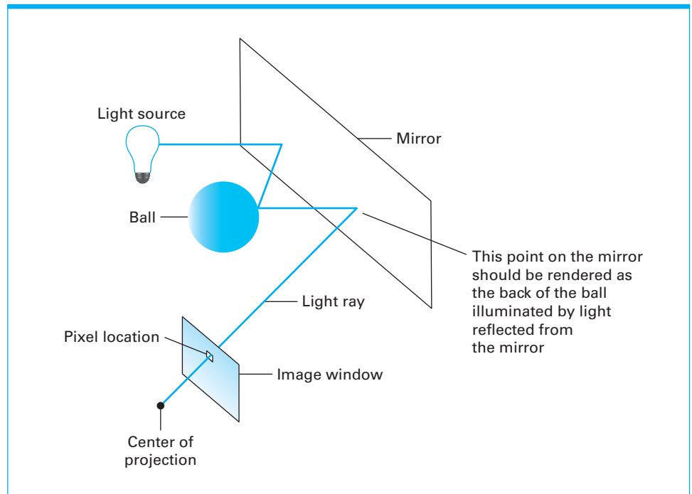
Figure 10.15 Ray tracing
