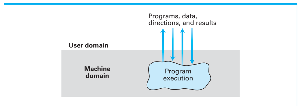
Figure 3.2 Interactive processing
